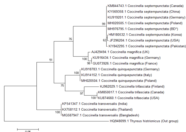
Fig. 2: Molecular Phylogenetic analysis by Maximum Likelihood method based on the nucleotide sequenc of COI gene. The evolutionary history was inferred using the Maximum Likelihood method based on the Tamura-Nei model. The tree was drawn to scale, with branch lengths measured in the number of substitutions per site. The percentage of trees in which the associated taxa clustered together was shown above the branches
