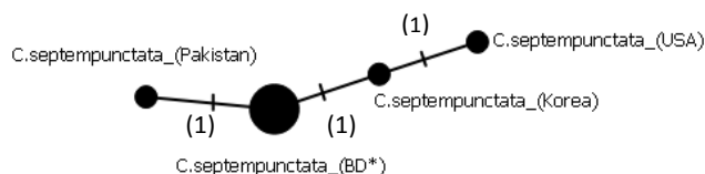
Fig. 1: Mitochondrial COI gene haplotype analysis of Coccinella septempunctata constructed by Popart1.7 based on TCS network. Big black circles represent the haplotype and small black circle represent the common ancestor. Mutational steps are presented by hatch marks and number
